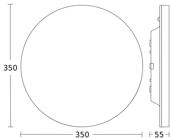
Dimension Drawing
